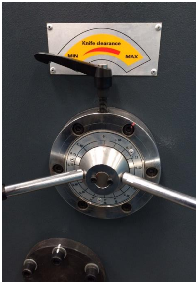
Blade gap adjustment
