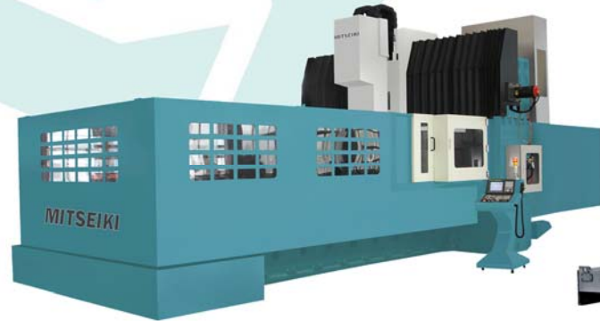
Mitseiki 2442A Double Column VMC Travels (X, Y, Z): 4200 x 2400 x 800mm, 4300 x 2000mm table, 16000kg table load, 32 tool side mount arm type ATC, BT50 spindle taper, 6000rpm spindle
