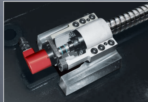
■ Precision Feedback System The semi-closed loop circuit system which the ball screw end is directly connected to the encoder ensures high positioning accuracy.
